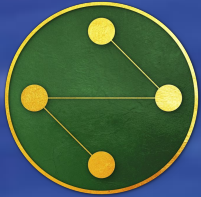
GENUS
