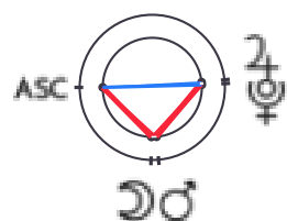
T-Square between Pluto in 29° Scorpio, Mars in 1° Virgo, Ascendant in 26° Taurus, Moon in 25° Leo, and Jupiter in 2° Sagittarius
